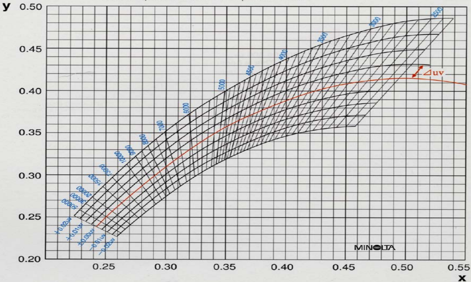
xy chromaticity chart indicating the black body locus, the isothermperature lines and equal \Delta uv lines.
